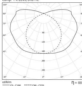
ECP 1x28W DC0 Lamp: 1 x 28W/840 HE
